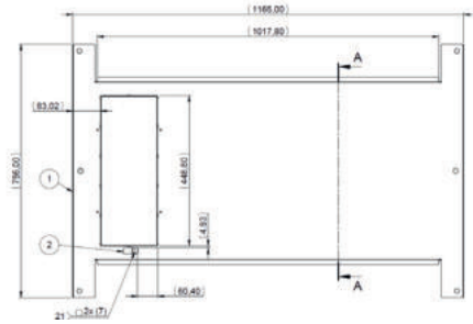
Cable entry top cover
