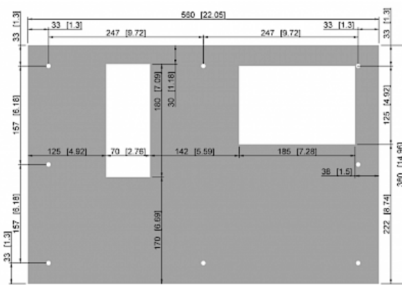
CUTOUT FOR EXTERNAL
