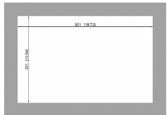
CUTOUT FOR INTERNAL / EXTERNAL
