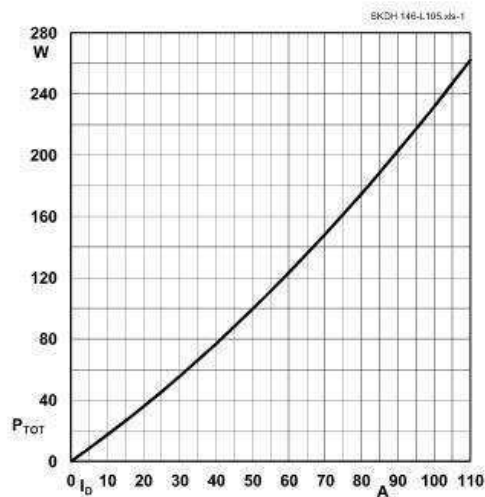
Fig. 1 Power dissipation per module vs. output current
