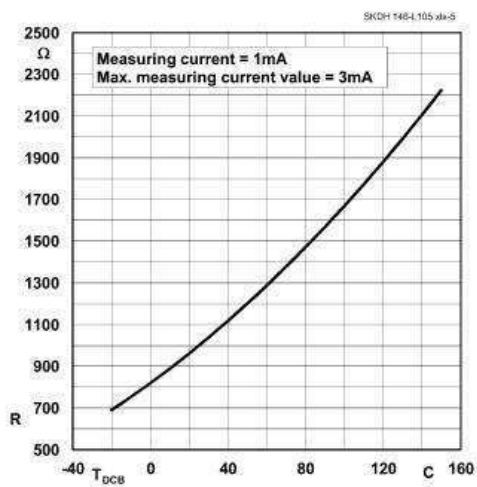
Fig. 5 Temperature sensor characteristic
