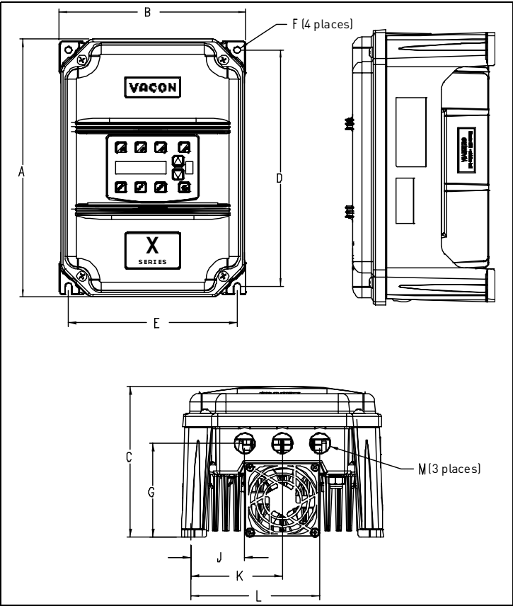
Figure 2: Vacon 50X Frame Size 1 Models
