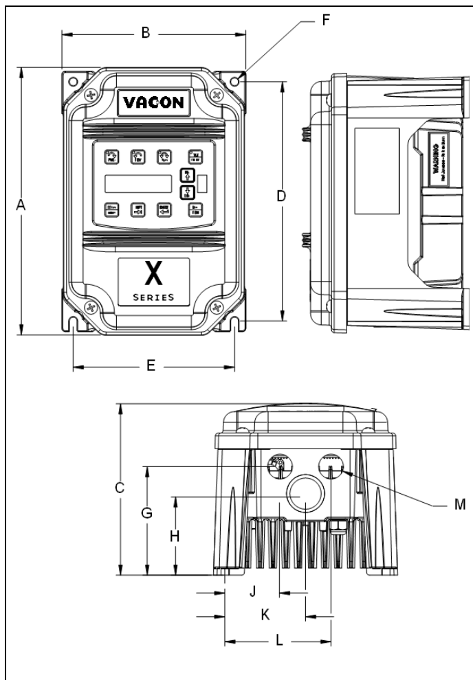
Figure 1: Vacon 50X Frame Size 0 Models
