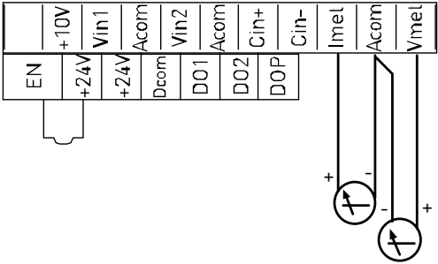
Figure 17: Connections for Process Meters
