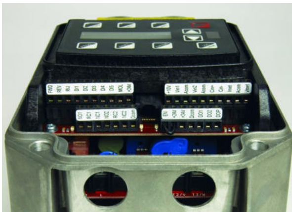
Figure 12: Vacon 50X Control Terminals
