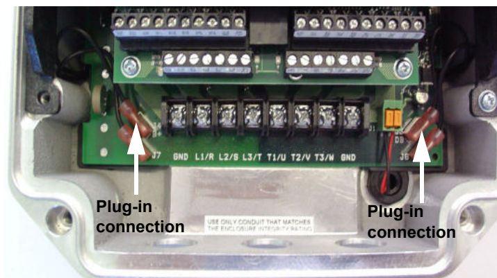
Figure 9: Power Terminals Size 1
