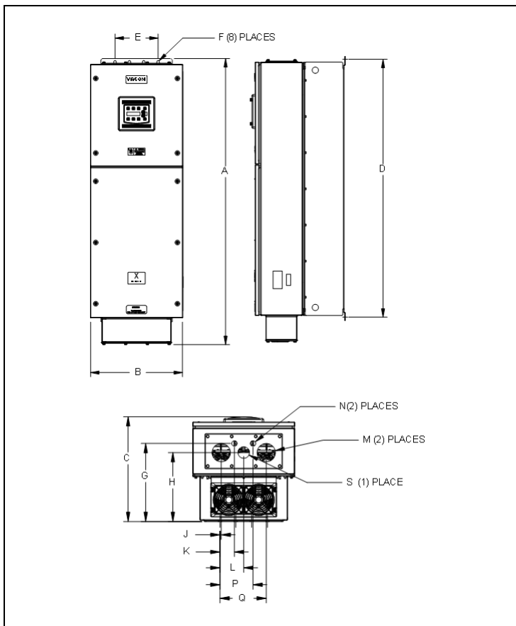
Figure 6: Vacon 50X Frame Size 5 Models
