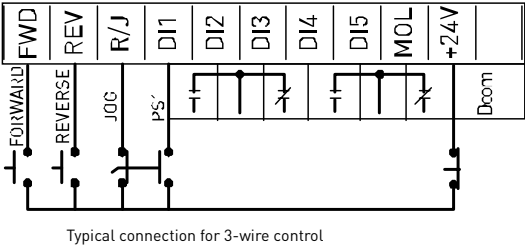
Figure 13: Connections for 2-wire and 3-wire Control
