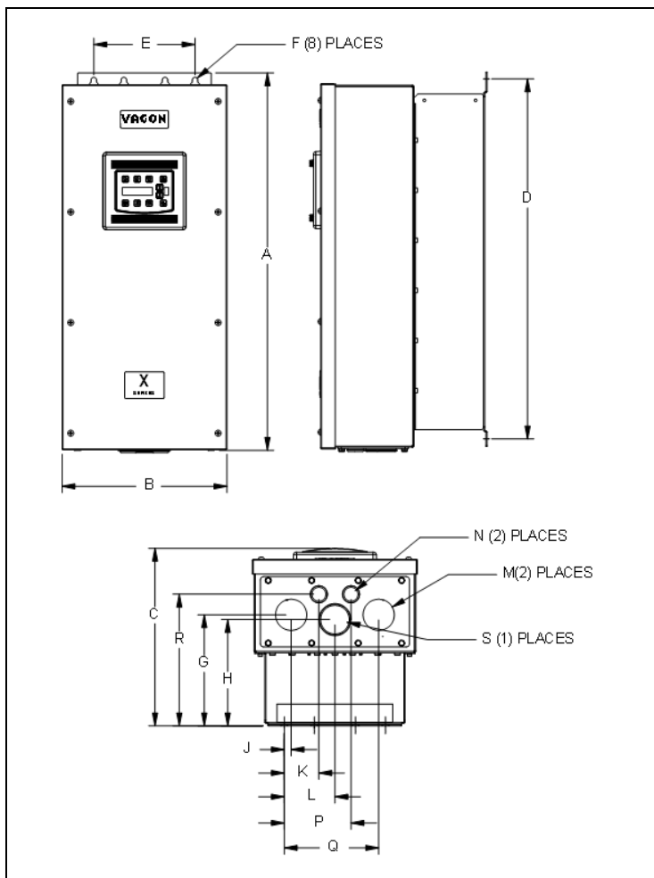
Figure 5: Vacon 50X Frame Size 4 Models
