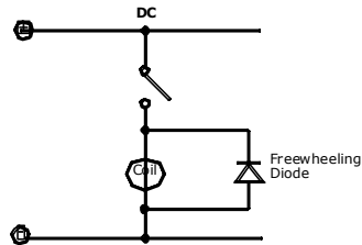
Figure 18: Connection Diagram for AC and DC Relay Coils and Solenoids
