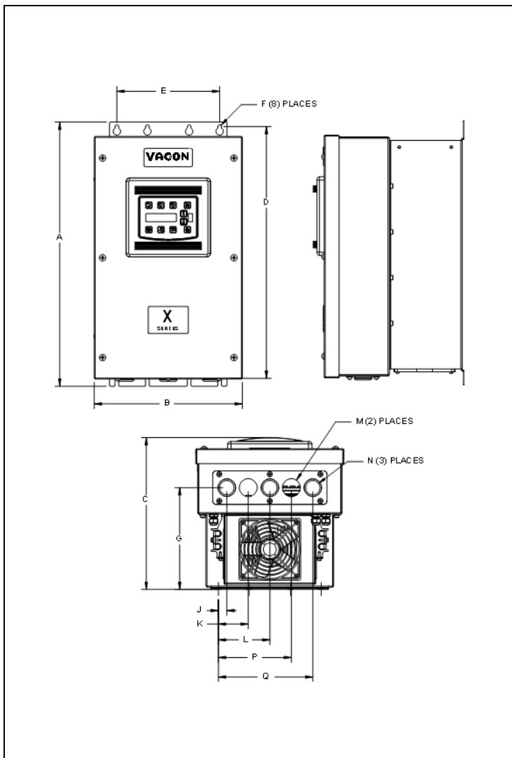
Figure 4: Vacon 50X Frame Size 3 Models
