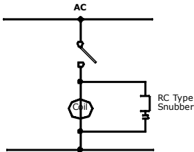
Figure 18: Connection Diagram for AC and DC Relay Coils and Solenoids
