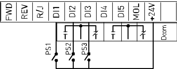
Figure 14: Connections for Preset Speeds
