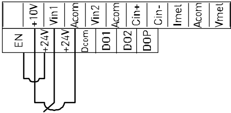
Figure 15: Connections for Speed Potentiometer
