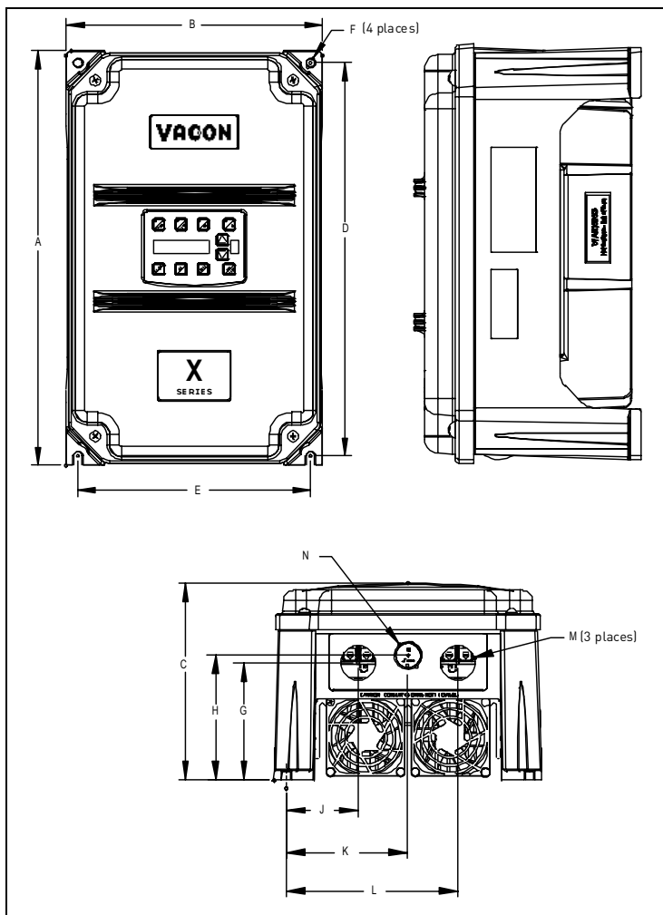
Figure 3: Vacon 50X Frame Size 2 Models
