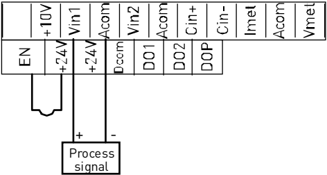
Figure 16: Connections for Process Signal
