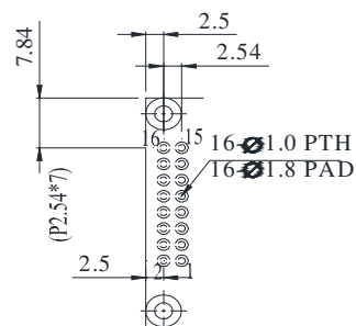
PIN DETAIL
