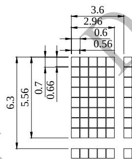
DOT SIZES SCALE 5/1
