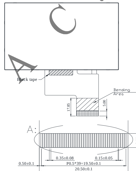
DETAIL A SCALE 4/1
