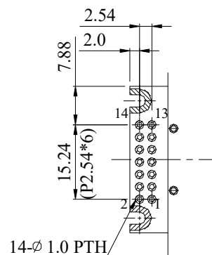
PIN DETAIL
