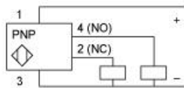
PNP 4-wire
