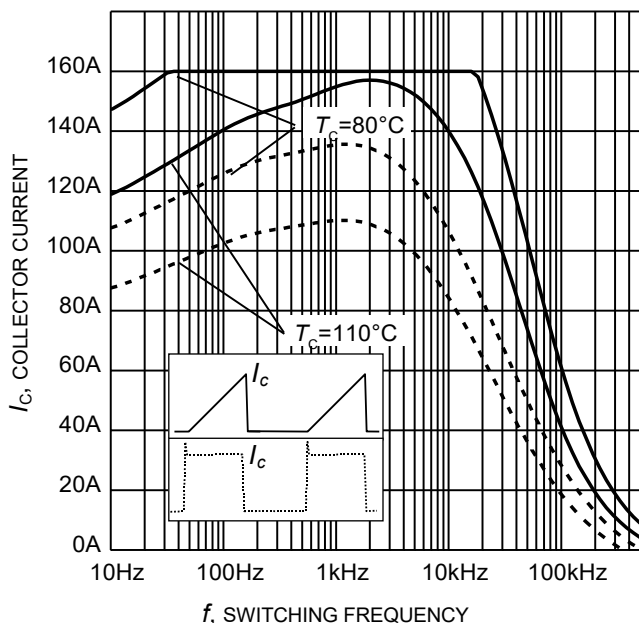
Figure 1. Collector current as a function of switching frequency ( T_j \leq 175^\circ\text{C} , D = 0.5 , V_{CE} = 600\text{V} , V_{GE} = 0/+15\text{V} , R_G = 12\Omega )
