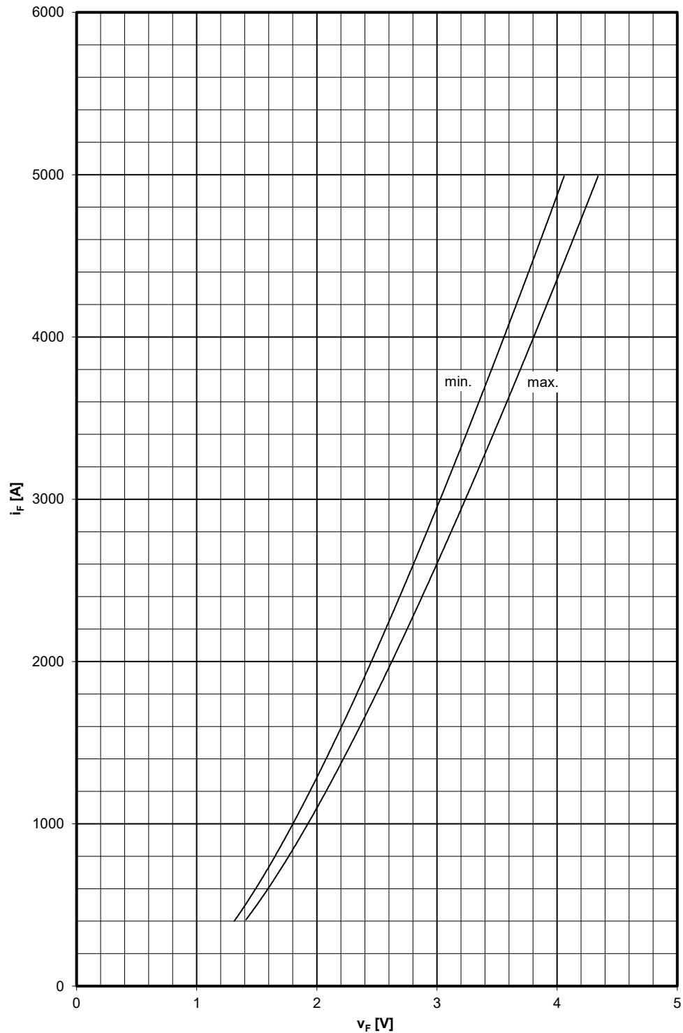
Grenzdurchlaßkennlinie / Limiting on-state characteristic i_F = f(v_F)
