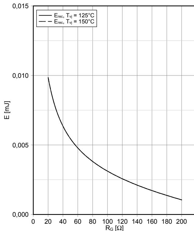
Schaltverluste Diode, 3-Level (typisch) switching losses Diode, 3-Level (typical) E_{rec} = f(R_G) I_F = 8\ \text{A} , V_{CE} = 300\ \text{V}
