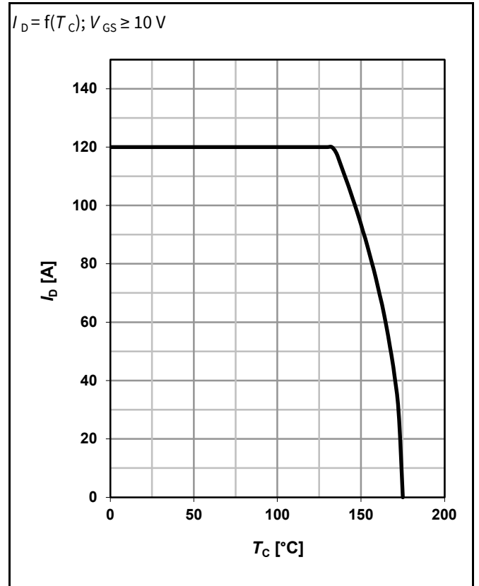
2 Drain current
