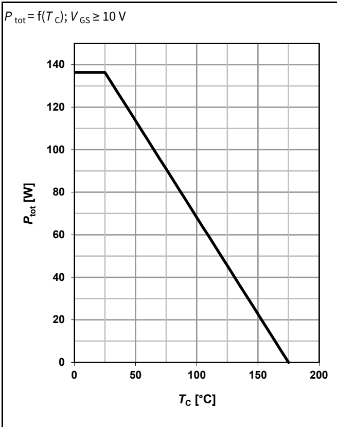
1 Power dissipation
