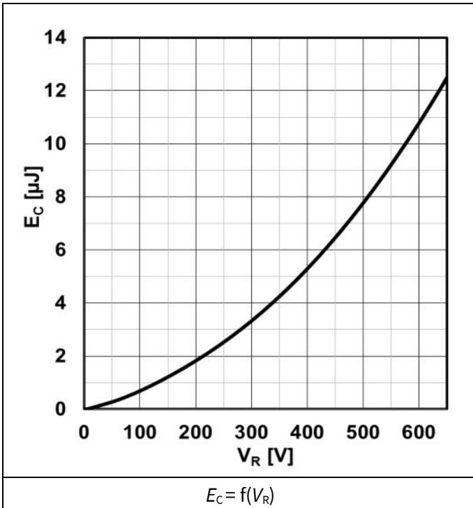
Figure 9 Typ. capacitance stored energy
