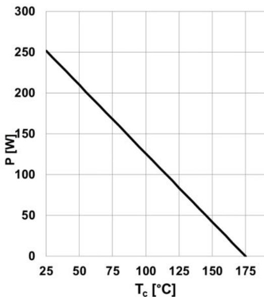
Figure 1. Power dissipation as function of case temperature, P_{\text{tot}}=f(T_c) , R_{\text{th(j-c)}}, \text{max}
