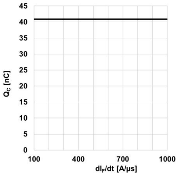
Figure 5. Typical capacitance charge as function of current slope 1 , Q_C=f(di/dt) , T_J=150^{\circ}\text{C} 1) Only capacitive charge, guaranteed by design.
