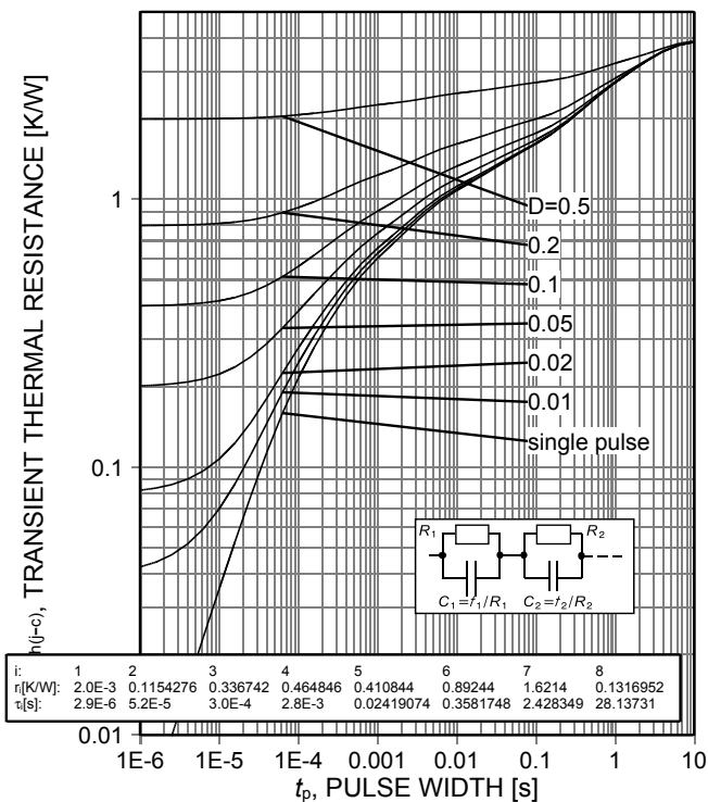
Figure 3. Diode transient thermal impedance as a function of pulse width ( D = t_p/T )
