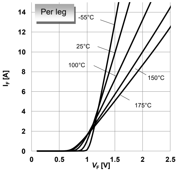
Figure 3. Typical forward characteristics per leg , I_F=f(V_F) , t_p=10\text{ }\mu\text{s} , parameter: T_j
