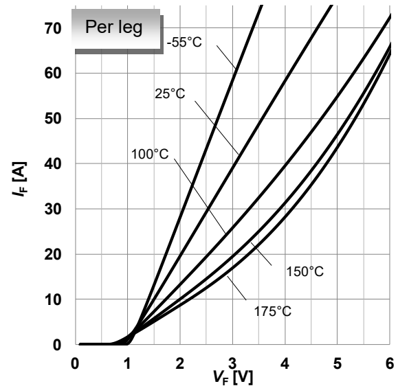
Figure 4. Typical forward characteristics in surge current per leg , I_F=f(V_F) , t_p=10\text{ }\mu\text{s} , parameter: T_j
