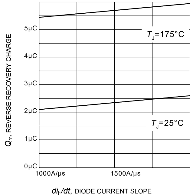
Figure 6. Typical reverse recovery charge as a function of diode current slope ( V_R = 400\text{V} , I_F = 75\text{A} , Dynamic test circuit in Figure E)
