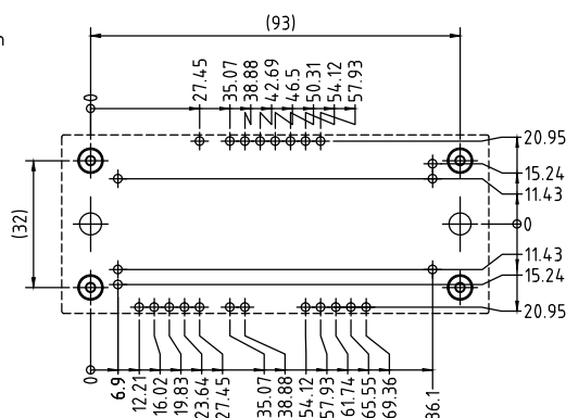
PCB hole pattern
