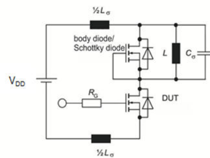
Figure E. Dynamic test circuit Parasitic inductance L_\sigma , parasitic capacitor C_\sigma ,
