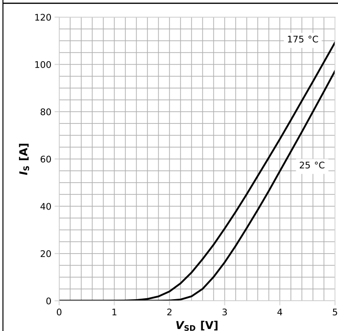
Diagram 13: Reverse output characteristics
