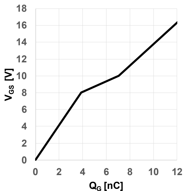
Figure 10 Typical gate charge ( V_{GS} = f(Q_G) , I_{DS} = 6A , V_{DS} = 800V , turn-on pulse)
