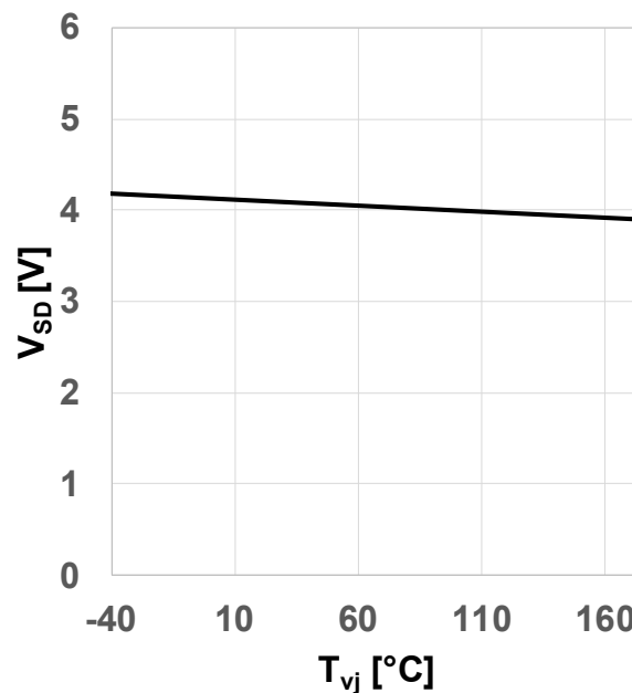
Figure 12 Typical body diode forward voltage as function of junction temperature ( V_{SD} = f(T_{vj}) , V_{GS} = 0V , I_{SD} = 6A )
