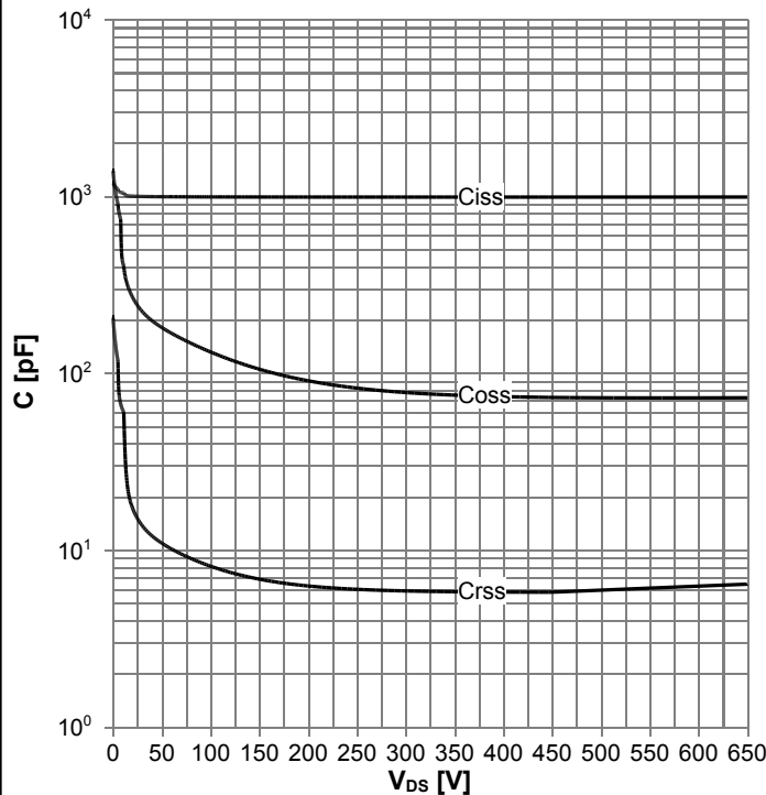
Diagram 15: Typ. capacitances
