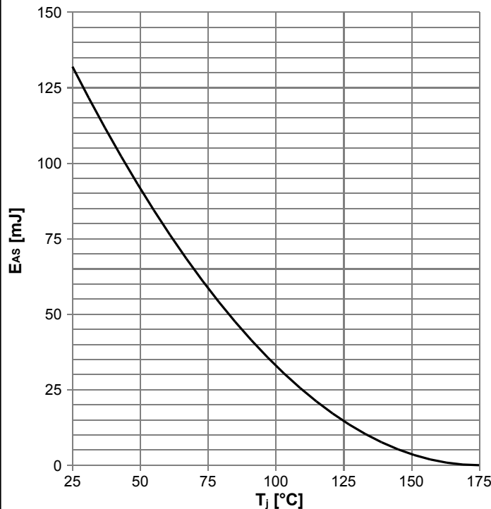
Diagram 13: Avalanche energy
