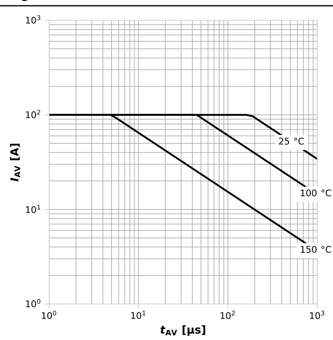
Diagram 14: Avalanche characteristics
