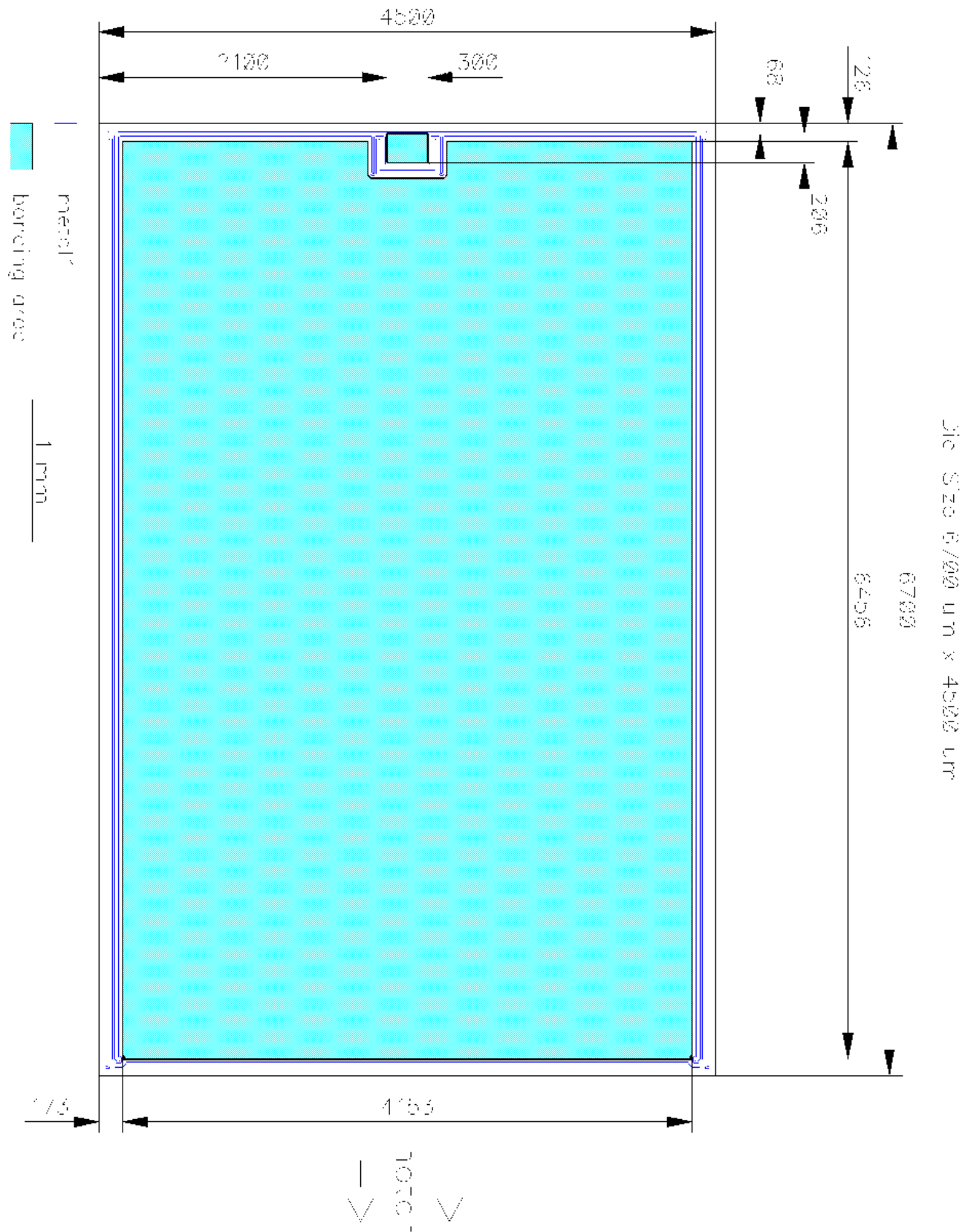
Figure 1 Outline Chip, dimensions in \mu\text{m}
