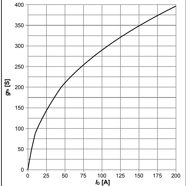
Diagram 8: Typ. transconductance
