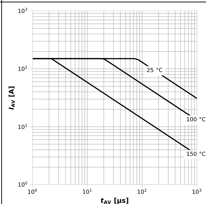
Diagram 14: Avalanche characteristics
