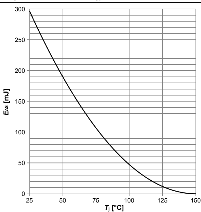
Diagram 12: Avalanche energy
