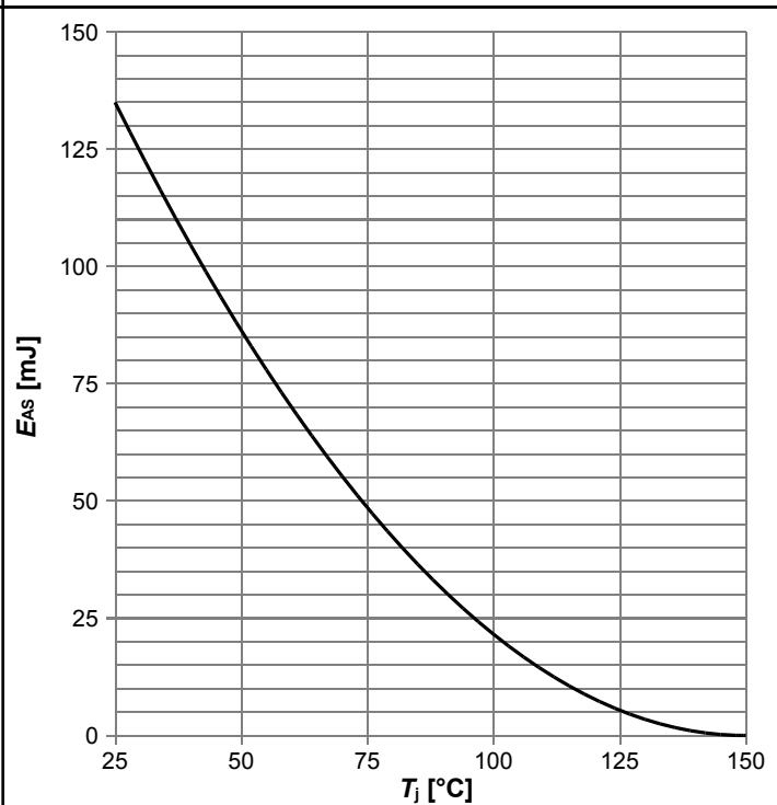
Diagram 12: Avalanche energy
