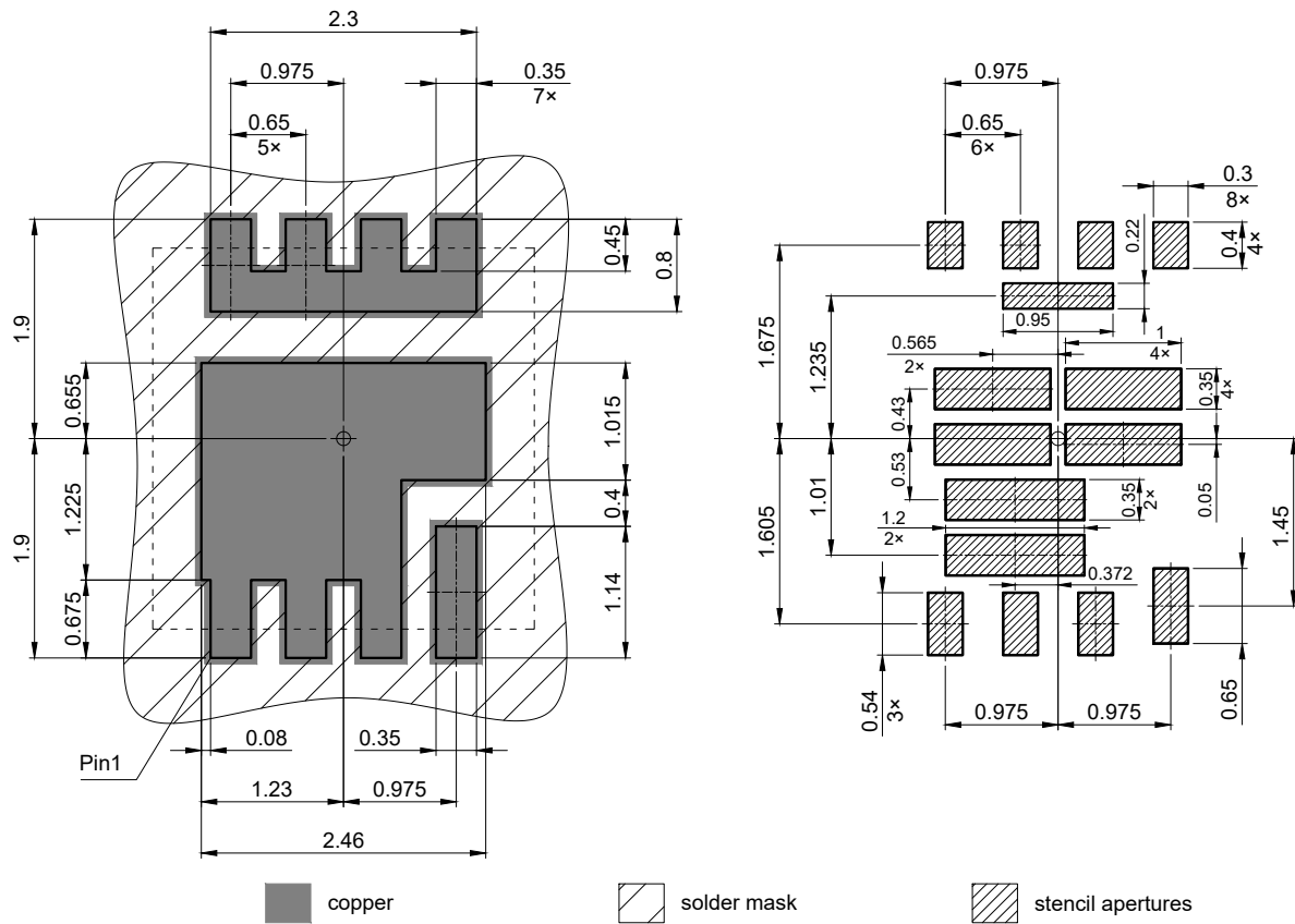
Figure 2 Outline Footprint (PG-WHSON-8-1), dimensions in mm
