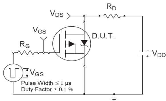
Fig 10a. Switching Time Test Circuit
