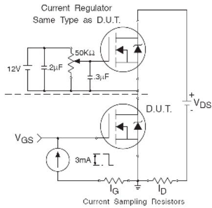
Fig 15a. Gate Charge Test Circuit
