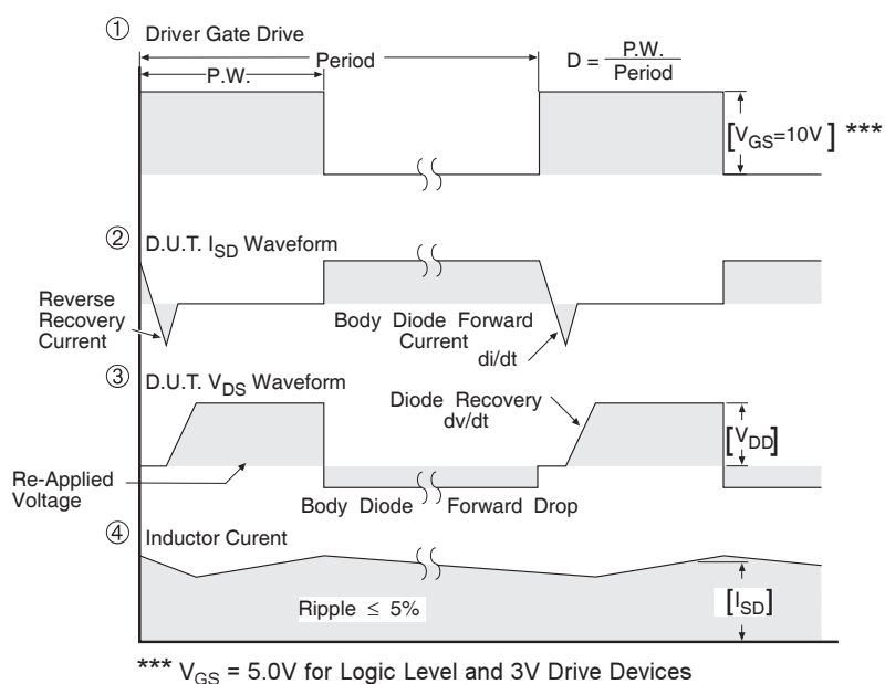
Fig 14. For P-Channel HEXFETS
