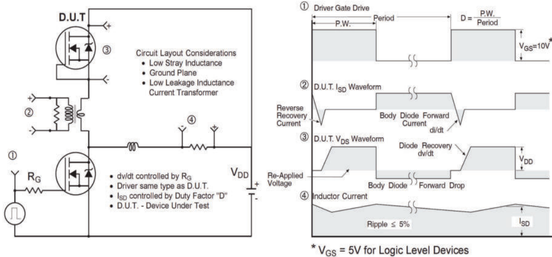
Fig 22. Peak Diode Recovery dv/dt Test Circuit for N-Channel HEXFET® Power MOSFETs
