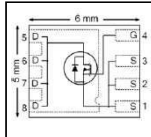
PQFN 5X6 mm
