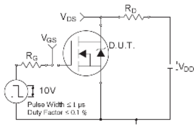
Fig 23a. Switching Time Test Circuit
