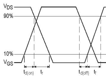
Fig 10b. Switching Time Waveforms
