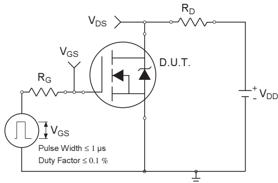
Fig 20a. Switching Time Test Circuit
