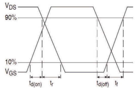
Fig 10b. Switching Time Waveforms
