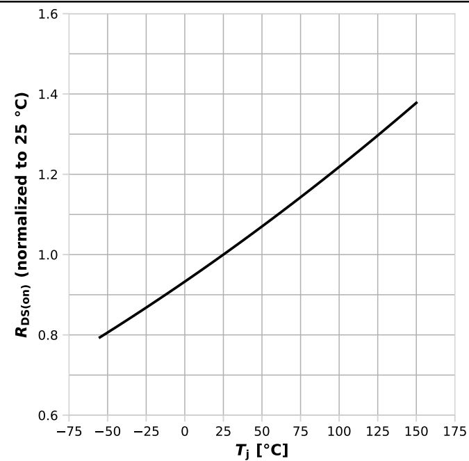
Diagram 24: Normalized drain-source on resistance (p-ch.)
