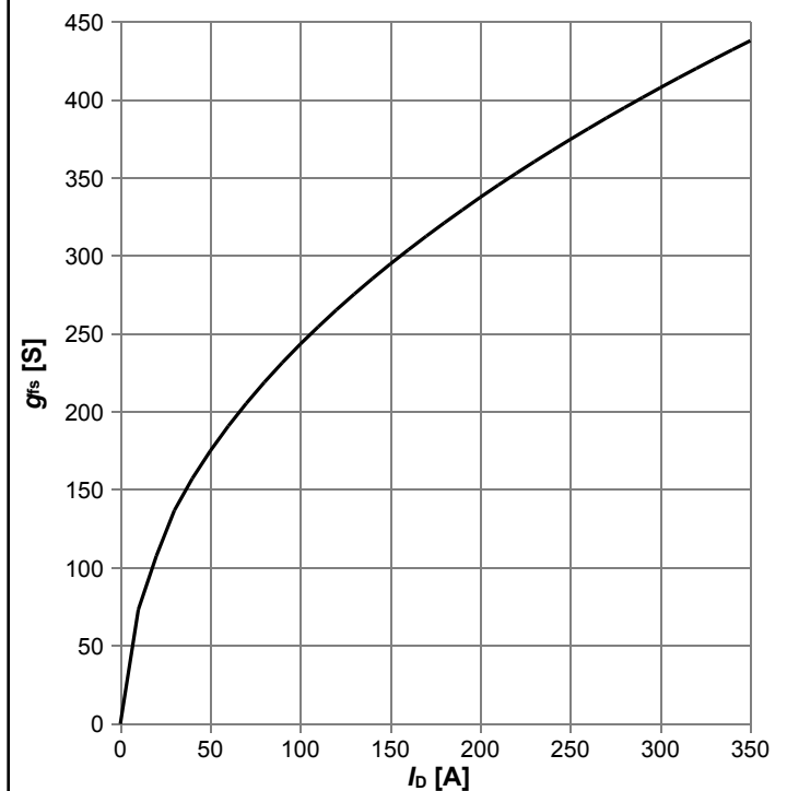
Diagram 8: Typ. transconductance
