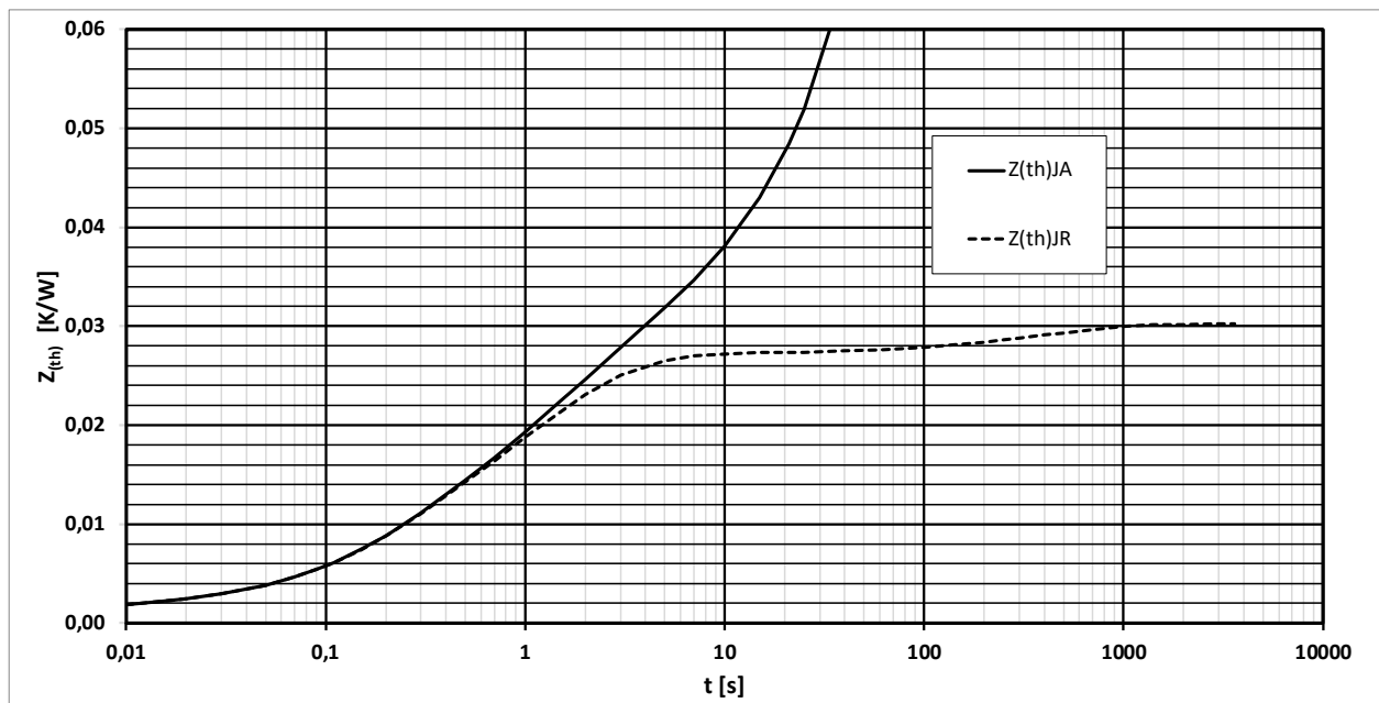
Transienter Wärmewiderstand je Zweig / Transient thermal impedance per arm Z_{thJR} = f(t) ; Z_{thJA} = f(t)
