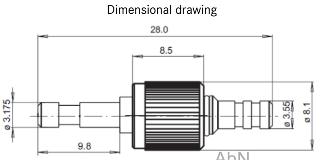
Knurl nut
