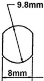
Mounting cutout
