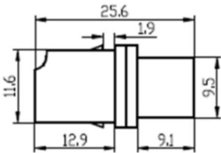
Coupling
