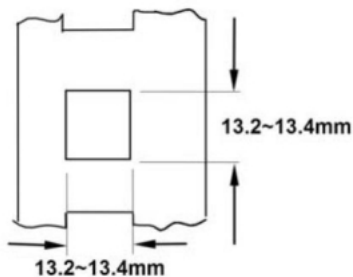
Mounting cutout
