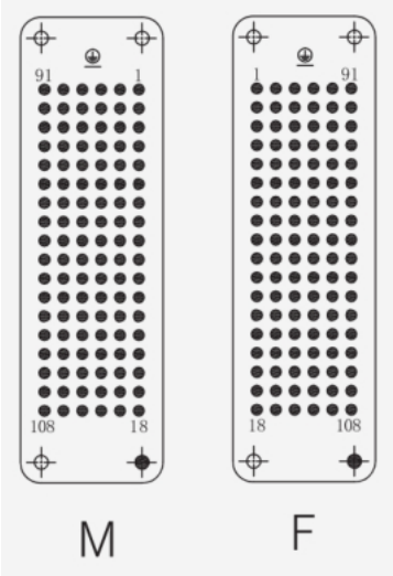
Pin assignment
